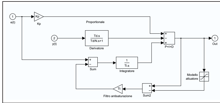
Figura 5.20: PID in Simulink a derivata limitata e anti-windup.
