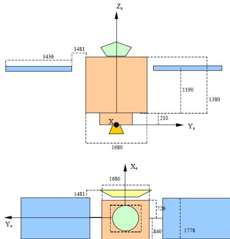
Figure 6-1: Satellite dimensions
