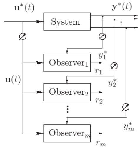
Output sensor FDI
