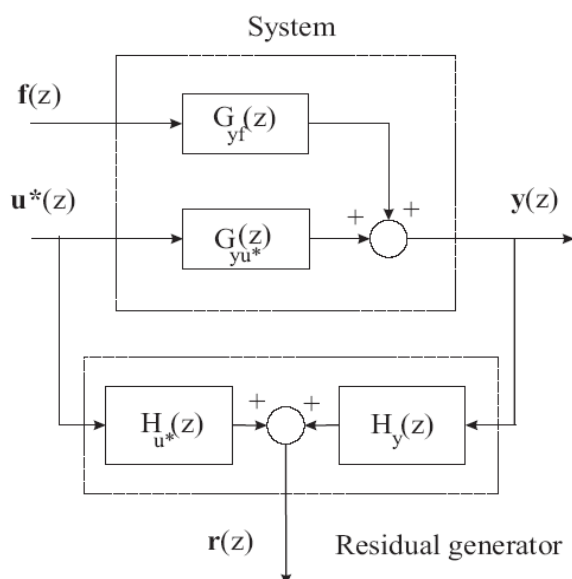
Figure 2.10: Residual generator general structure. 24/09/2020
