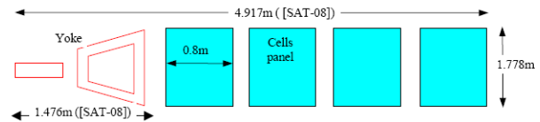
Figure 6-2: MARS-EXPRESS solar array
