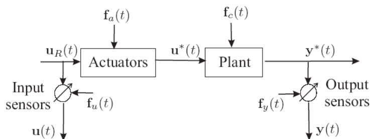
Figure 2.7: Fault topology with actuator input signal measurement.
