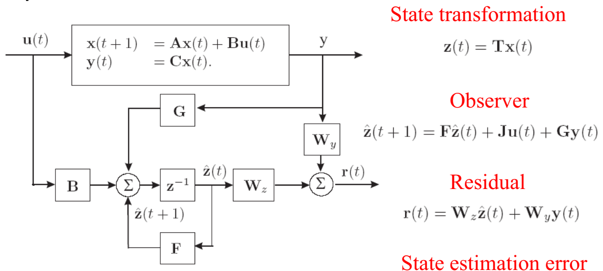
Figure 2.15: Process and output observer. \mathbf{e}_x(t) = \hat{\mathbf{z}}(t) - \mathbf{z}(t) = \hat{\mathbf{z}}(t) - \mathbf{T}\mathbf{x}(t)
