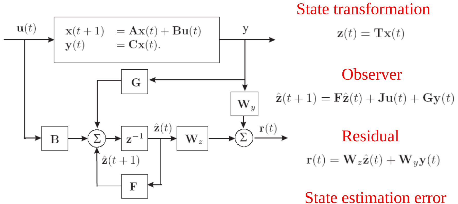
Figure 2.15: Process and output observer.
