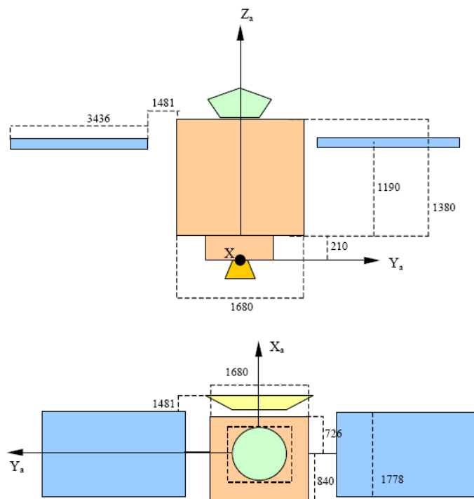
Figure 6-1: Satellite dimensions
