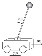
Figure 3.5: Inverted pendulum
