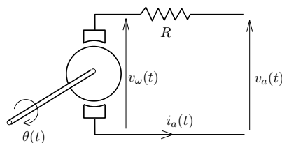
Figure 3.2: Simplified model of a d.c. motor
