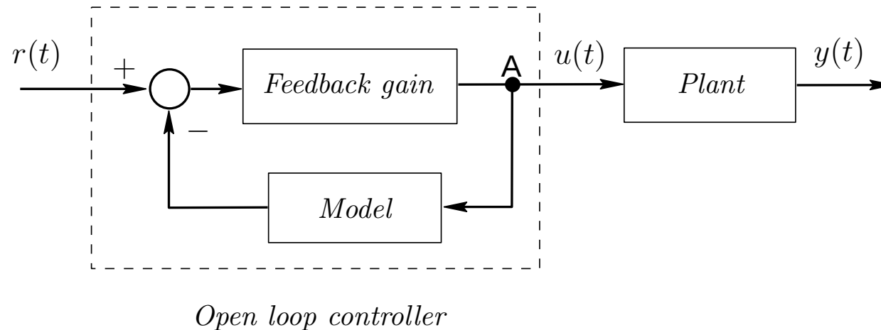
Figure 2.9: Open loop controller
